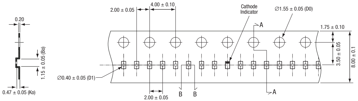
Figure 11. SOD-882 Package Dimension Drawing
