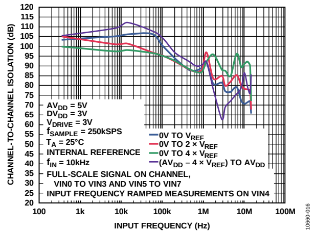
Figure 15. ADC Channel-to-Channel Isolation
