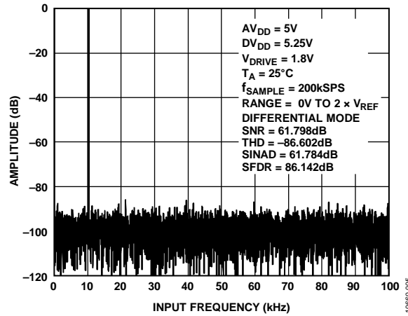
Figure 7. ADC FFT, 200 kSPS, f_{IN} = 10 kHz, Differential Mode
