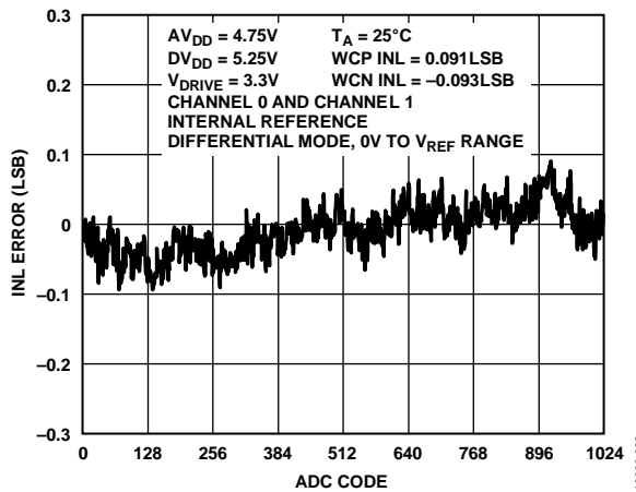
Figure 8. Typical ADC INL, Differential Mode
