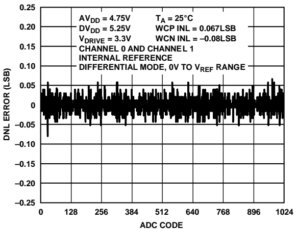
Figure 9. Typical ADC DNL, Differential Mode
