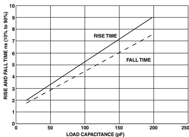
Figure 77. Typical Rise and Fall Times (10% to 90%) vs. Load Capacitance for Driver B at V_{DDEXT} = 3.65\text{ V}
