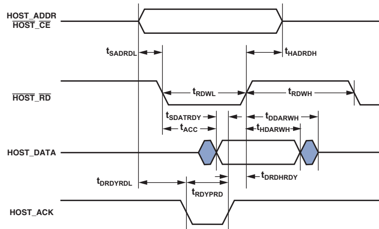
Figure 45. HOSTDP A/C—Host Read Cycle
