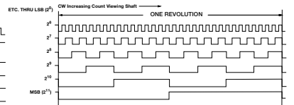
Figure 2 Natural Binary
