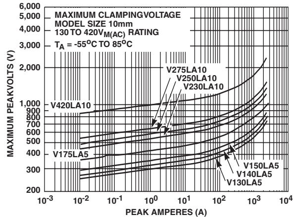
FIGURE 6. CLAMPING VOLTAGE FOR V130LA5 - V420LA10
