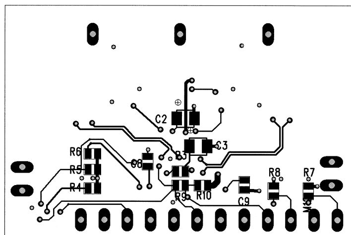
FIGURE 3. Bottom Layer
