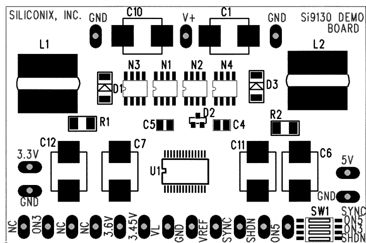
FIGURE 1. Top Silkscreen
