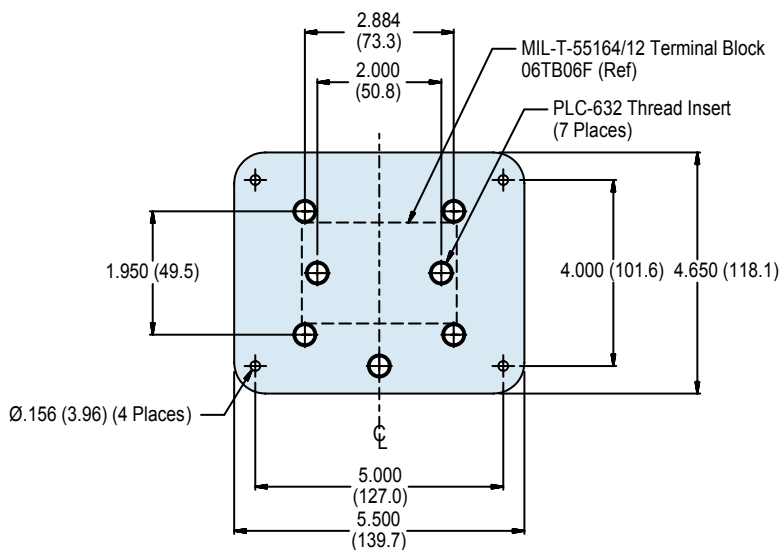
DETAIL B
