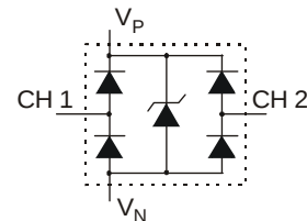
Device Schematic
