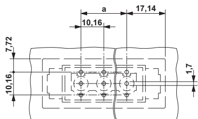
Drilling diagram
