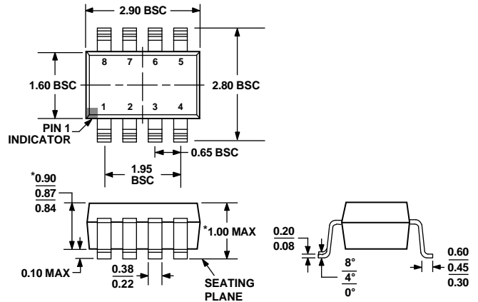
Figure 36. 8-Lead Thin Small Outline Transistor Package [TSOT] (UJ-8) Dimensions shown in millimeters
