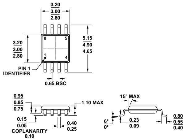
COMPLIANT TO JEDEC STANDARDS MO-187-AA Figure 35. 8-Lead Mini Small Outline Package [MSOP] (RM-8) Dimensions shown in millimeters
