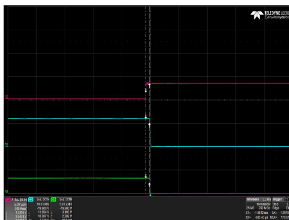
Figure 12: DS1600SPE-3 Turn Off Characteristic via PS_KILL_L Full Load: I_o = 129.8\text{A} , I_{sb} = 3.5\text{A} Ch 2: PS_KILL_L Ch 3: Vo Ch 4: Pwr_Good
