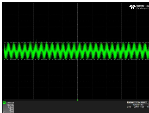
Figure 10: DS1600SPE-3 Ripple and Noise Measurement – V_{in} = 180\text{Vac} Full Load: I_o = 129.8\text{A} , I_{sb} = 3\text{A} Ch 4: Vo
