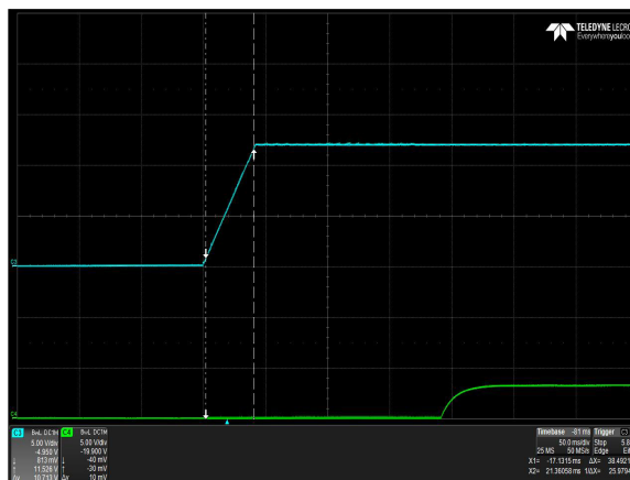
Figure 8: DS1600SPE-3 Output Voltage Startup – V_{in} = 180\text{Vac} Full Load: I_o = 129.8\text{A} , I_{sb} = 3.5\text{A} Ch 3: Vo Ch 4: Pwr_Good
