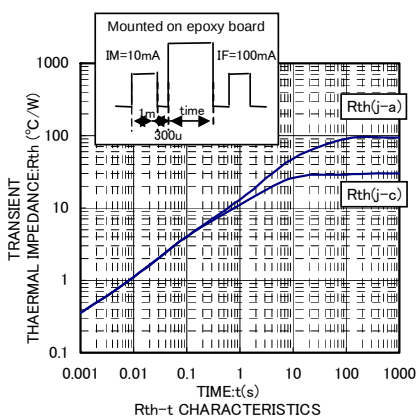
Rth-t CHARACTERISTICS
