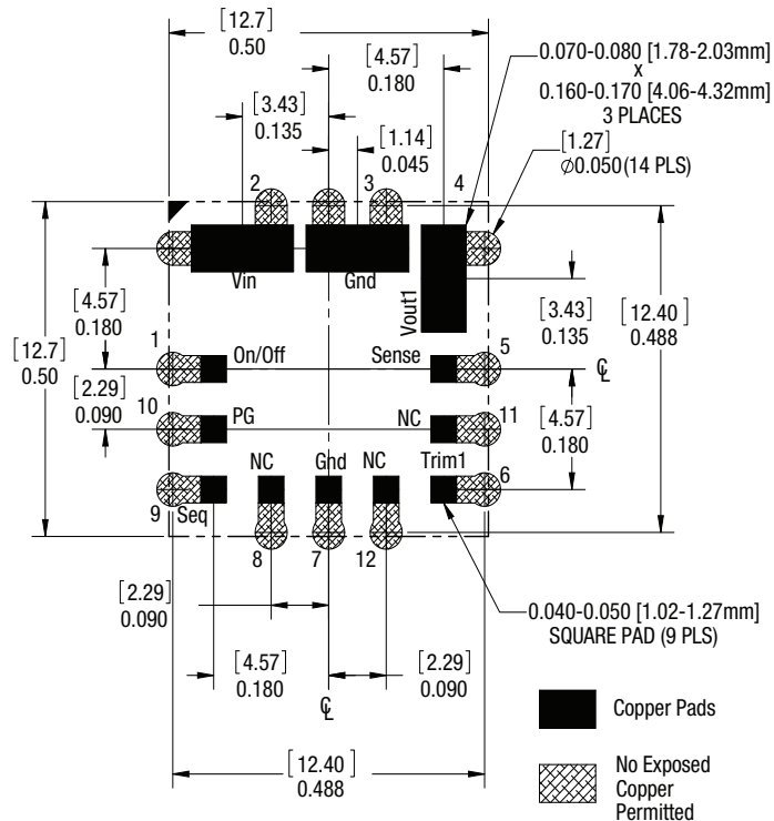
Figure 3. OKL-T/6-W12 Mechanical Outline
