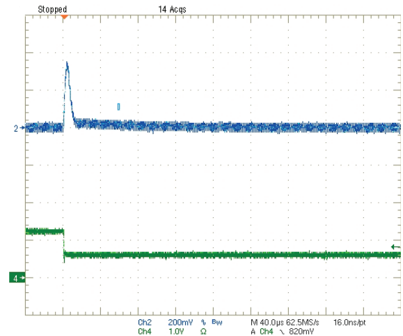
Step Load Transient Response (Vin=12V, Vout=3.3V, Load=0, Iout=6A to 3A) Trace 2=Vout, 200 mV/div. Trace 4=Iout, 5A/div.
