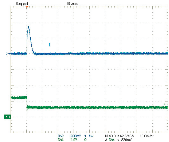
Step Load Transient Response (Vin=12V, Vout=.591V, Load=0, Iout=6A to 3A) Trace 2=Vout, 200 mV/div. Trace 4=Iout, 5A/div.
