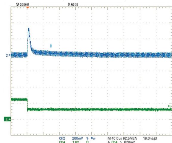
Step Load Transient Response (Vin=12V, Vout=5.0V, Load=0, Iout=6A to 3A) Trace 2=Vout, 200 mV/div. Trace 4=Iout, 5A/div.
