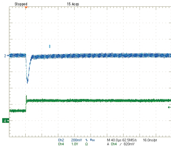
Step Load Transient Response (Vin=12V, Vout=3.3V, Cload=0, Iout=3A to 6A) Trace 2=Vout, 200 mV/div. Trace 4=Iout, 5A/div.
