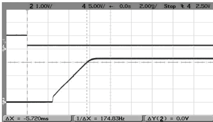
On/Off Enable Delay (Vin=12V, Vout=3.3V, Iout=6A, Cload=0) Trace 4=Enable, Trace 2=Vout
