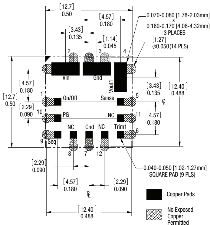
Recommended Footprint -through the Board-
