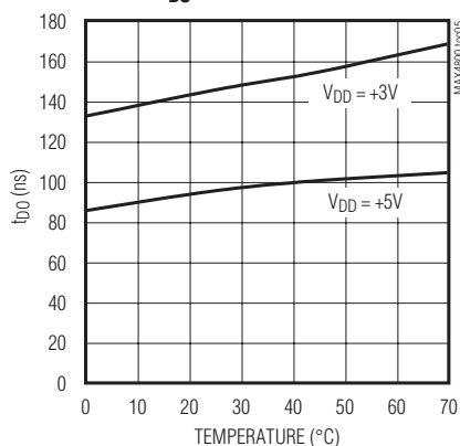
t_{PD} vs. TEMPERATURE
