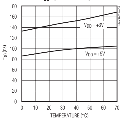
t_{PD} vs. TEMPERATURE
