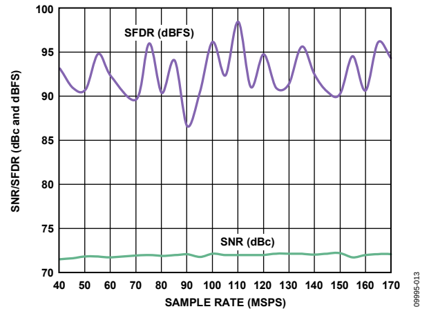
Figure 14. AD9642-170 Single-Tone SNR/SFDR vs. Sample Rate ( f_s ) with f_{IN} = 90 MHz
