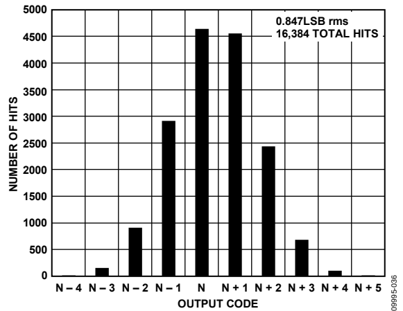
Figure 39. AD9642-250 Grounded Input Histogram, f_s = 250 MSPS
