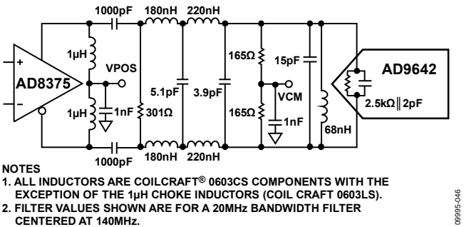
Figure 49. Differential Input Configuration Using the AD8375
