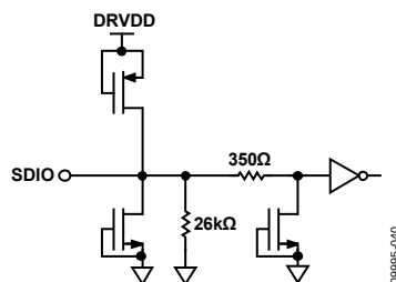
Figure 43. Equivalent SDIO Circuit
