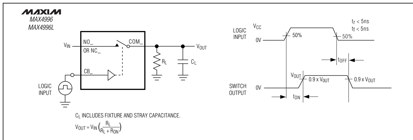
Figure 1. Switching Time
