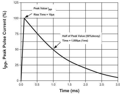
10x1,000 \mu s Surge Current Waveform
