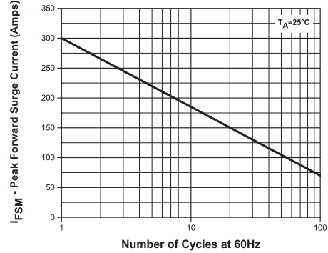
Maximum Non-Repetitive Peak Forward Surge Current
