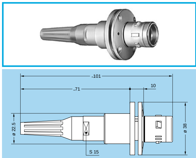
FMW.3K Fixed plug with round flange (4 holes fixing), keys (W), cable adapter, with bend relief
