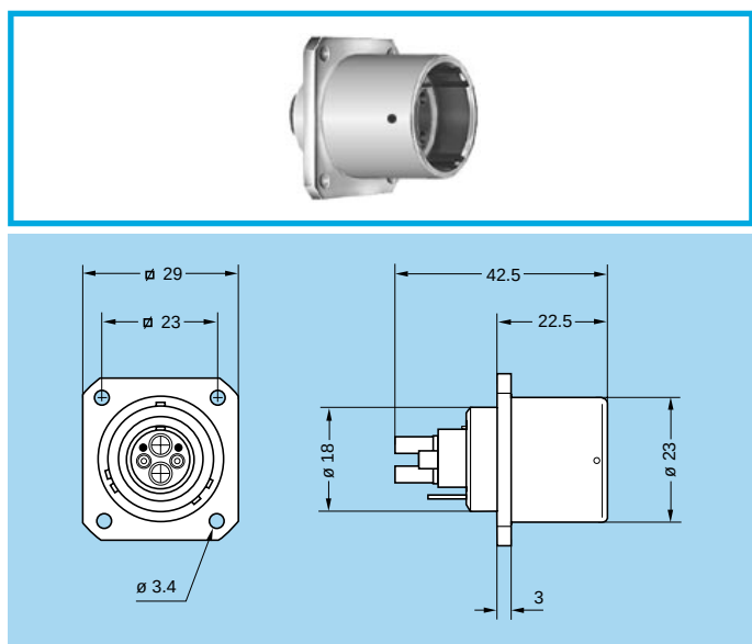
EDW.3K Fixed socket with rear square flange (4 holes fixing), keys (W), and earthing tag
