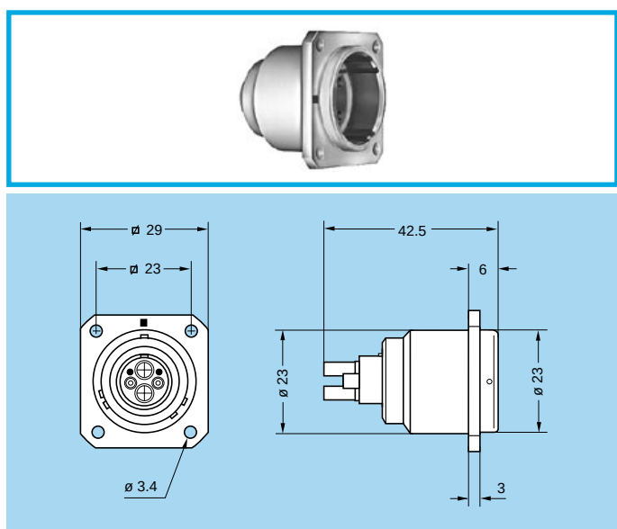
EBW.3K Fixed socket with front square flange (4 holes fixing), keys (W)
