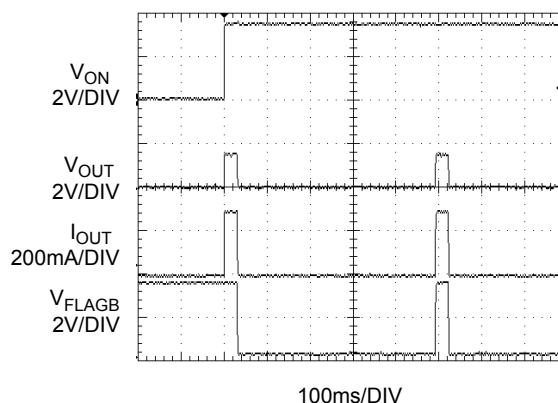
Figure 16. T_{RESTART} Response
