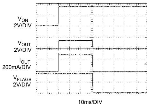
Figure 15. T_{BLANK} Response
