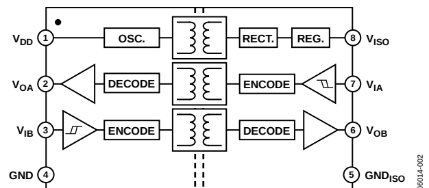
Figure 2. ADuM5241
