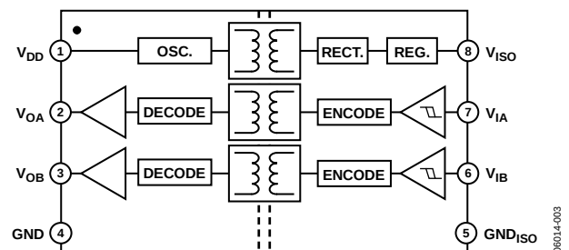
Figure 3. ADuM5242
