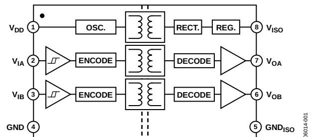
Figure 1. ADuM5240
