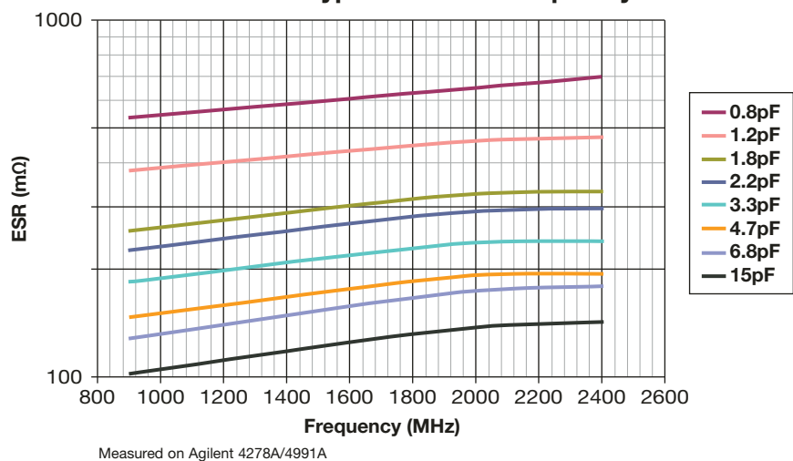
Accu-P® 0201 Typical ESR vs Frequency
