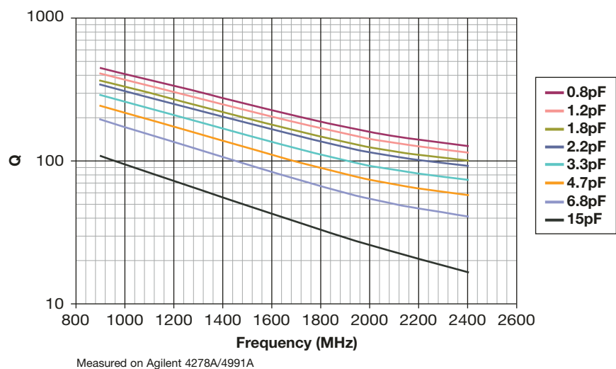
Accu-P® 0201 Typical Q vs Frequency
