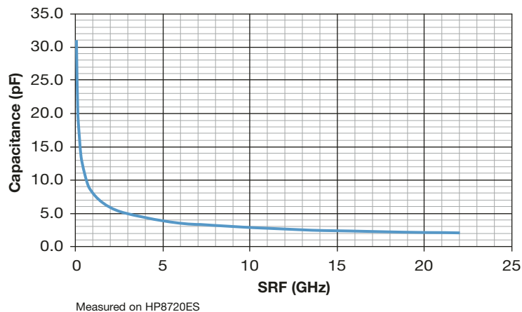
Accu-P® 0201 Typical SRF vs Capacitance
