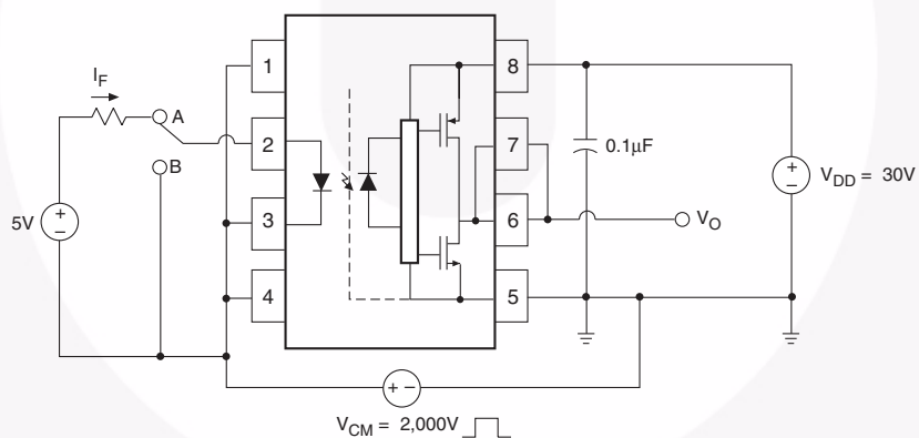
Figure 29. t_{PLH} , t_{PLH} , t_r and t_f Test Circuit and Waveforms
