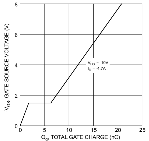
Figure 10 Gate-Charge Characteristics
