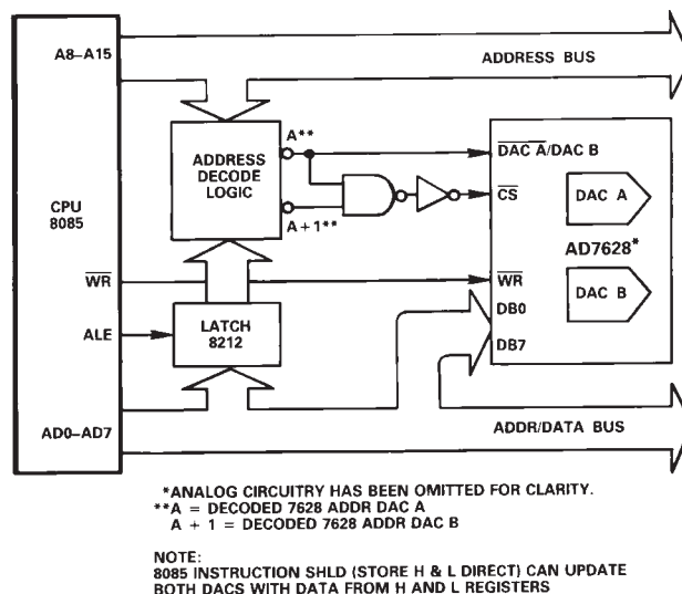
Figure 12. AD7628 Dual DAC to 8085 CPU Interface
