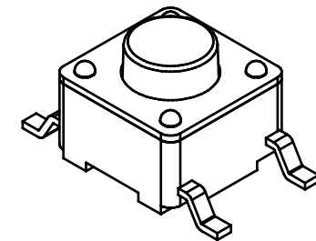
ISOMETRIC
