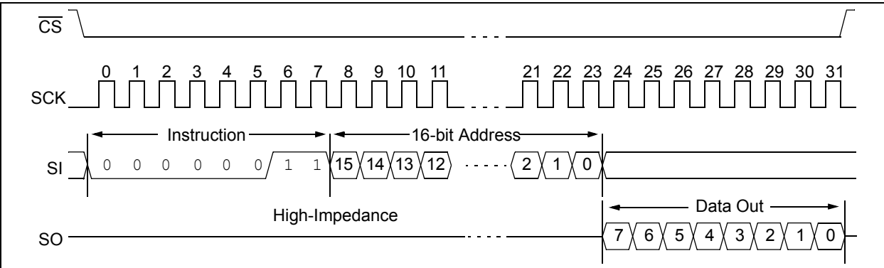
FIGURE 2-1: READ SEQUENCE
