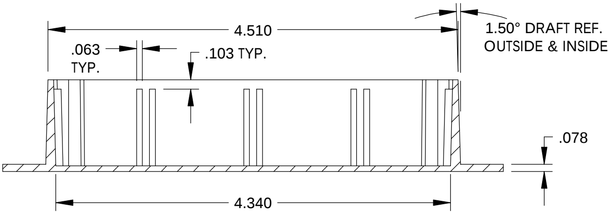
SECTION B-B
