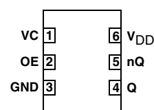
IDT8N4SV75 6-lead ceramic 5mm x 7mm x 1.55mm package body CD Package Top View
