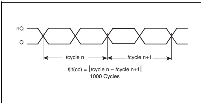
Cycle-to-Cycle Jitter
