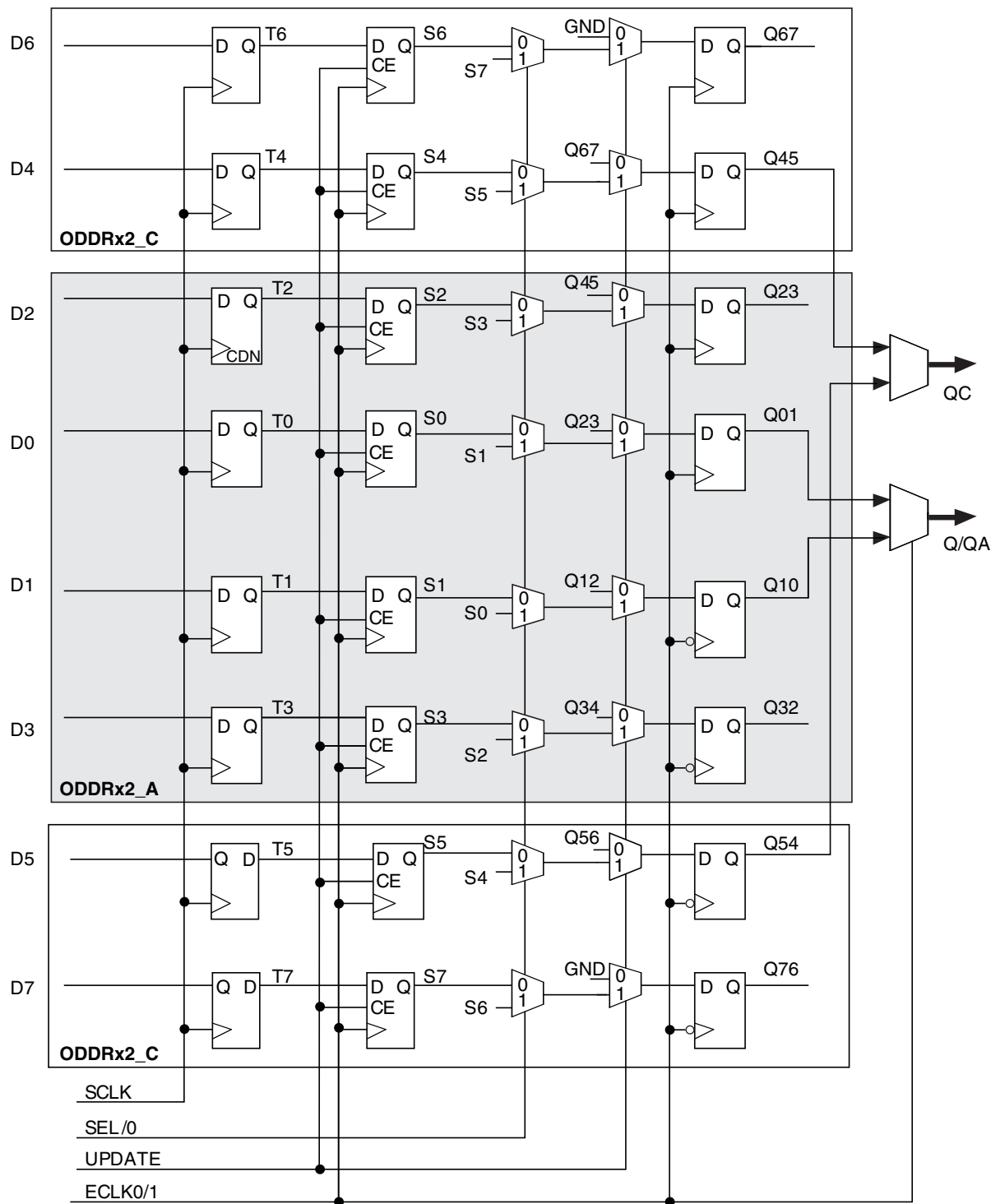
Figure 2.14. Output Gearbox
