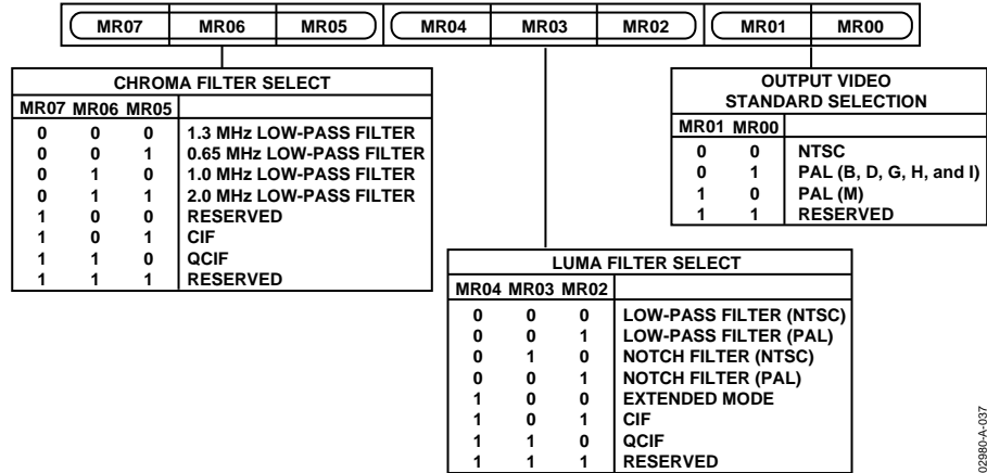
Figure 38. Mode Register 0
