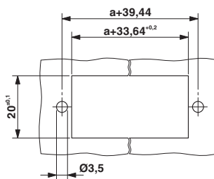
Sheet metal cutout for screw connection.
