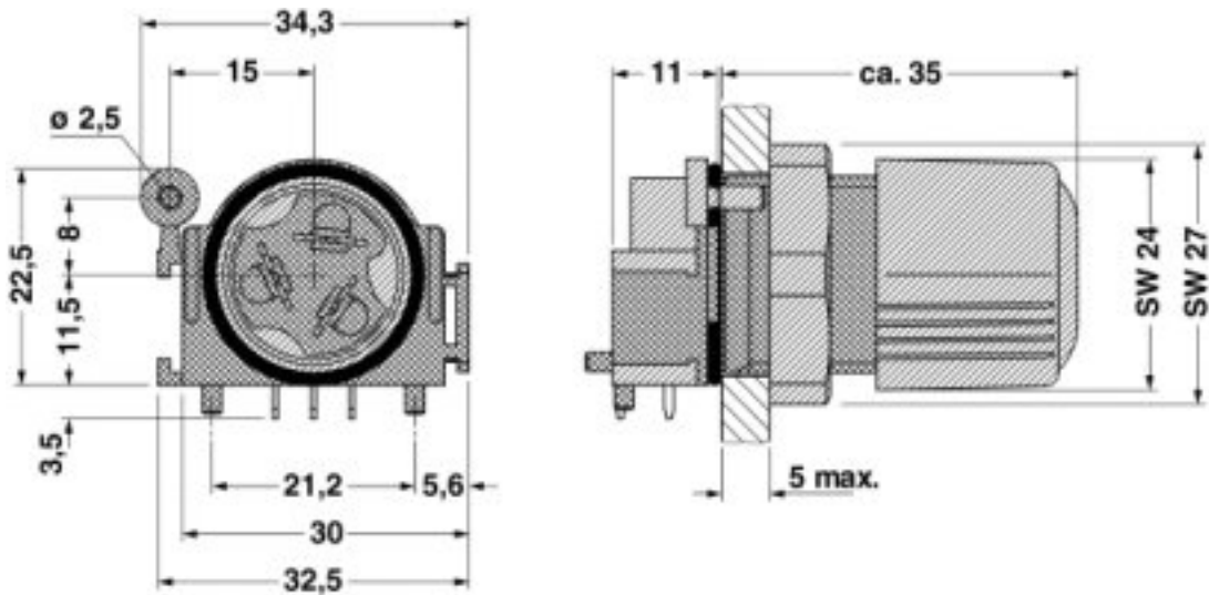
Dimensioned drawing
