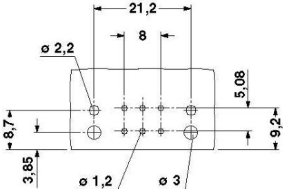
Dimensioned drawing
