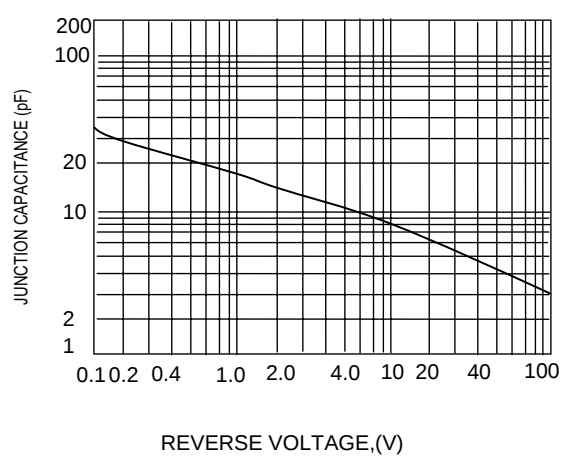
TYPICAL CAPACITANCE
