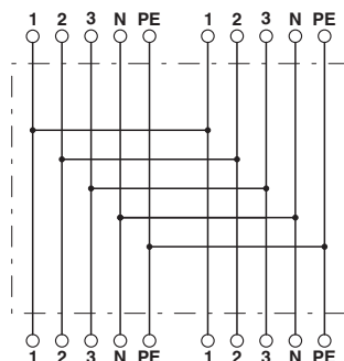
Circuit diagram
