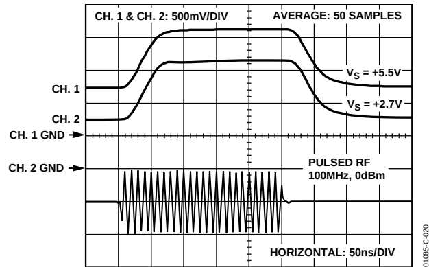
Figure 19. Response Time, No Signal to 0 dBm
