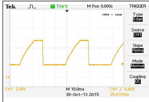
FIGURE 8-4: BOOST V_{\text{PP}} 6V TO 18V AND DISCHARGE 18V TO 6V; DISCHARGE ON, V_{\text{DD}} = 3.3\text{V} , \text{CVPP}(\text{C2}) = 10\text{ }\mu\text{F}
