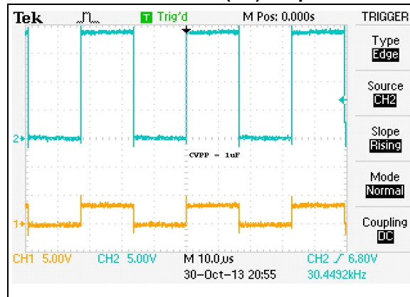
FIGURE 8-3: OE vs. OUT00; V_{\text{DD}} = 3.3\text{V} , V_{\text{PP}} = 18\text{V} , \text{CVPP}(\text{C2}) = 1\text{ }\mu\text{F}
