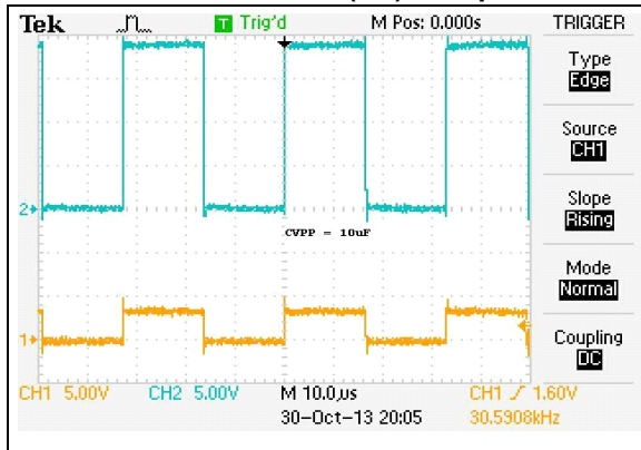
FIGURE 8-2: OE vs. OUT00; V_{\text{DD}} = 3.3\text{V} , V_{\text{PP}} = 18\text{V} , \text{CVPP}(\text{C2}) = 10\text{ }\mu\text{F}
