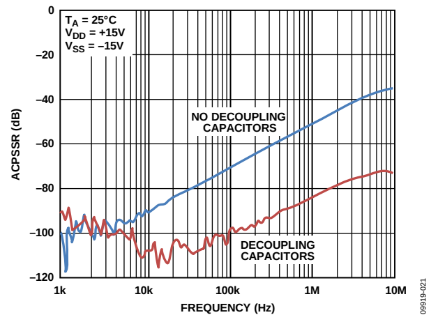
Figure 22. ACPSSR vs. Frequency, \pm 15 V Dual Supply
