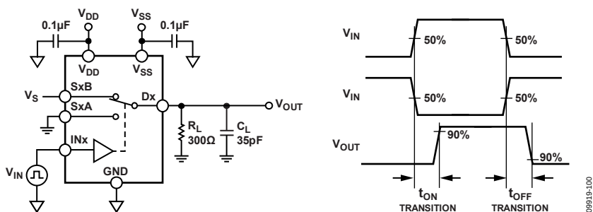
Figure 33. Switching Timing
