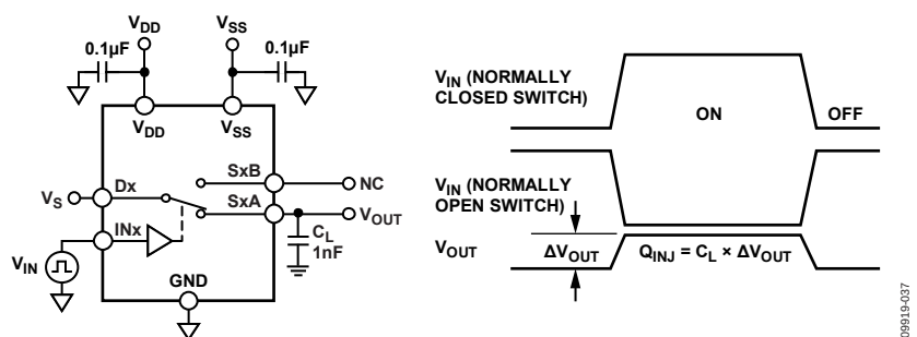
Figure 36. Charge Injection
