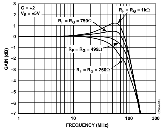
Figure 14. AD8130 Frequency Response for Various R_F/R_C
