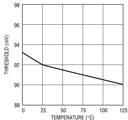
Current Limit Amplifier CL1 Threshold
