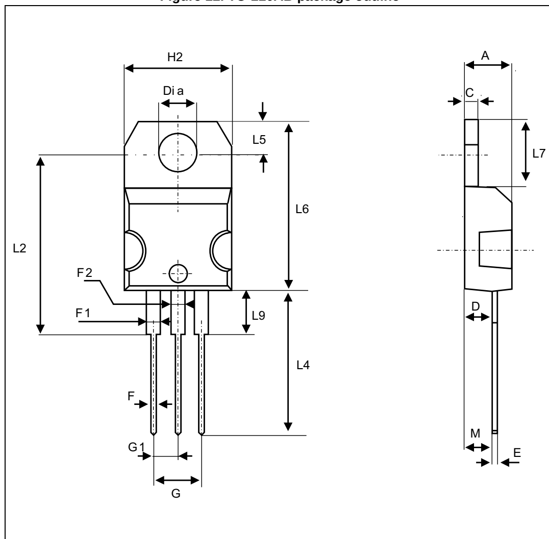
Figure 12. TO-220AB package outline
