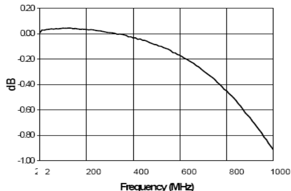
Amplitude Imbalance
