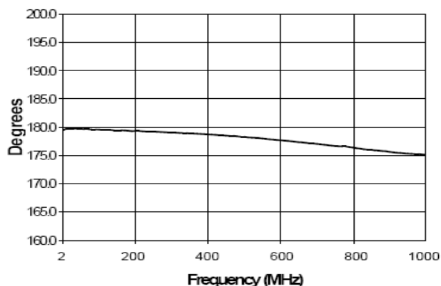
Phase Imbalance
