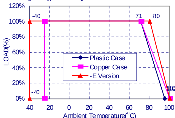
Figure1. Typical Derating curve for Natural Convection
